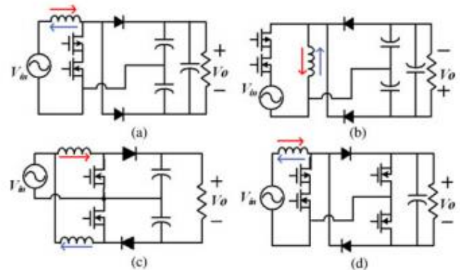
Fig. 2: Split capacitor topology (a) split capacitor boost converter. (b) Split capacitor buck boost converter. (c) Two switch boost converters. (d) Boost converter with secondary switch. [4]
