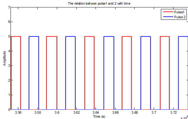
Fig 16: Pulse (1) and pulse (2) with 25% width and 10µs time delay
